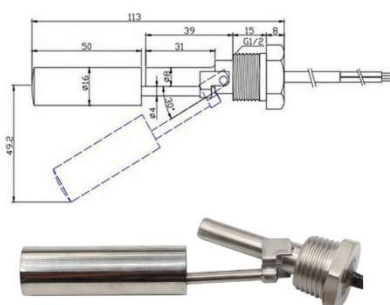
Float type level switch
