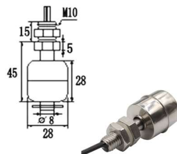
Magnetic float switch
