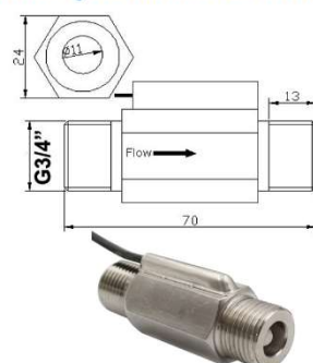
Electronic metal paddle flow switch
