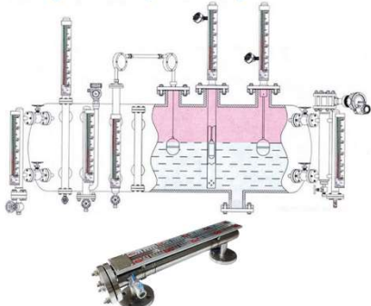
Oil Magnetic Float Liquid Level Gauge Remote Control
